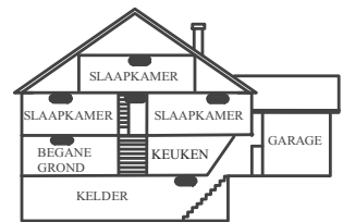
● KOOLMONOXIDEDETECTOR
